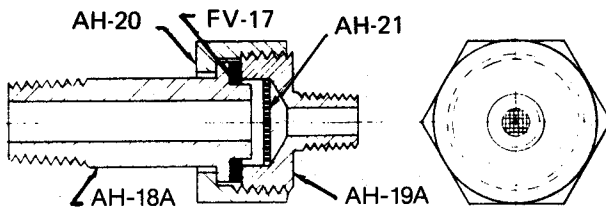
STRAINER UNION ASSEMBLY AH-17
